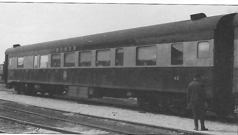
◀ OMI #AF-1053 Monon Rebuilt Coach #46, 7 lg windows on left side, stainless grille and 8 lg windows on right side, f/p black/ gold, lettered, lights, interior, interior lights.
